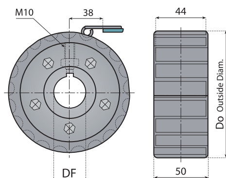
整体式主动轮 (注塑) SINGLE PIECE SPROCKET (INJECTION)
