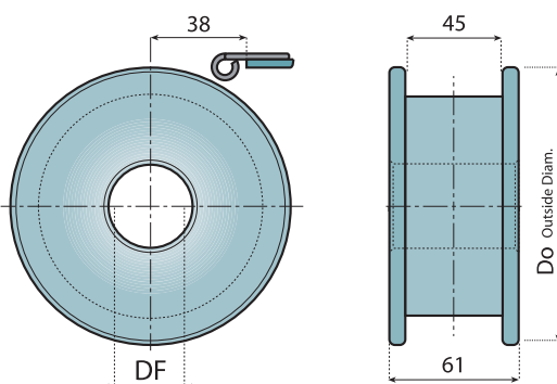
整体式从动轮 (机加工) SINGLE PIECE IDLER WHEEL ( MACHINED )
