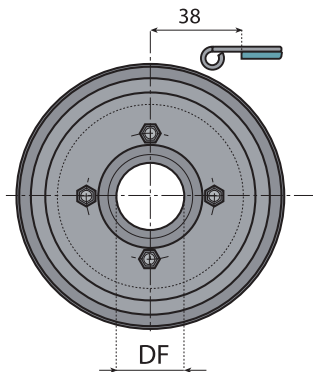
从动轮 (注塑) IDLER WHEEL (INJECTION)
