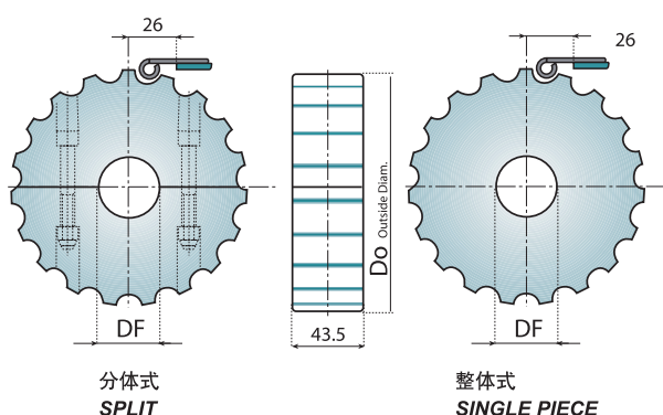
适用于 512-515 链条 FOR CHAIN 512-515
