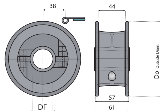
分体式从动轮 (注塑) SPLIT IDLER WHEEL ( INJECTION )
