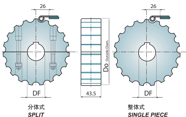
适用于 512-515 链条 FOR CHAIN 512-515
