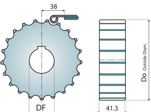
整体式主动轮 (机加工) SINGLE PIECE SPROCKET (MACHINED)
