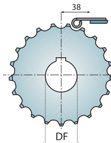
整体式 SINGLE PIECE
